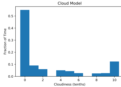
Figure 1. The distribution of cloudiness as measured at CTIO. We model the observatory as closed for cloud levels above 3/10.
