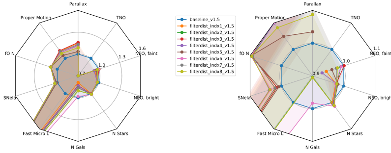
Figure 10. Science impact of varying the filter distribution
