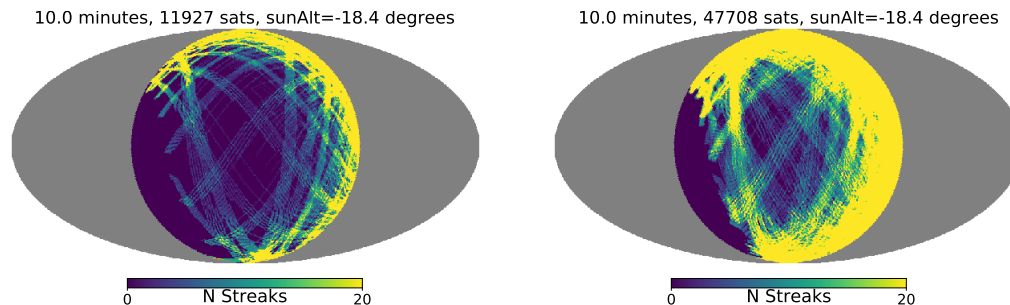
Figure 41. Alt/az projection of simulated satellite megaconstellations as seen from the Rubin Observatory site after twilight has ended.
