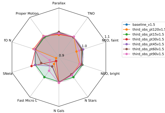
Figure 17. The science impact of dedicating the end of the night to gathering observations of areas that already have pairs.
