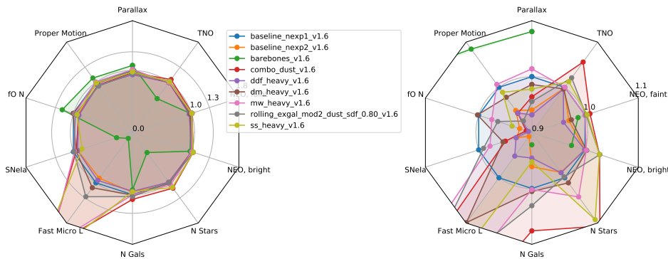
Figure 40. Science impact for the v1.6 runs. The barebones survey performs very well on SRD requirements at the expense of almost all other science. The combo_dust run is the opposite, with low SRD scores and high science performance.
