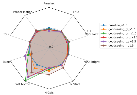
Figure 13. The science impact of making sure the sky has template images in good seeing conditions.
