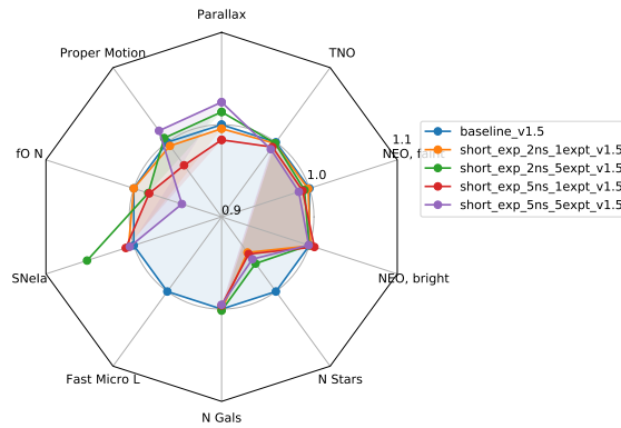
Figure 15. Science impact of covering the sky in short exposures.
