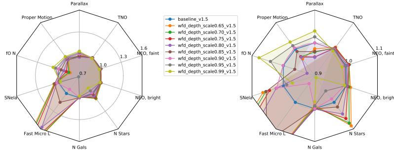
Figure 23. The Science impact of varying the WFD depth.
